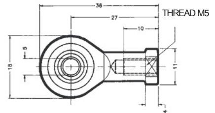
BALLJOINT SF
