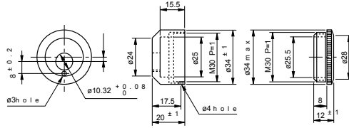
Adaptor A (without lock device)
